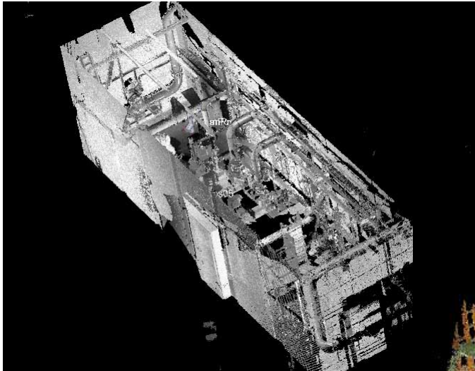
3D-Intensity-Histogram
